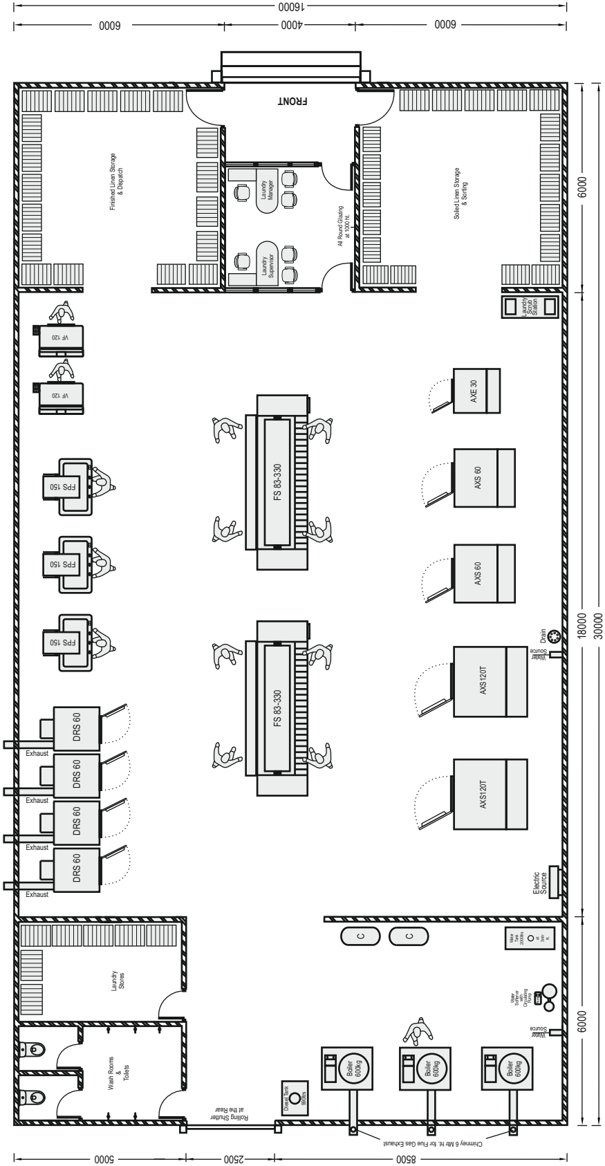
This is a Typical Layout that may be altered or modified to suit a particular requirement. Recommended Clear Height : 5 mtrs.
